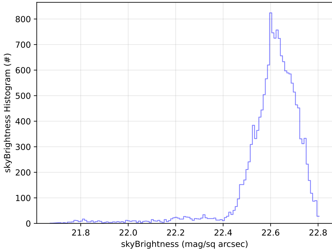
ddf_acor_sf10_lsf40_lsr20_v3.4_10yrs Yr 1 u band: skyBrightness Histogram
