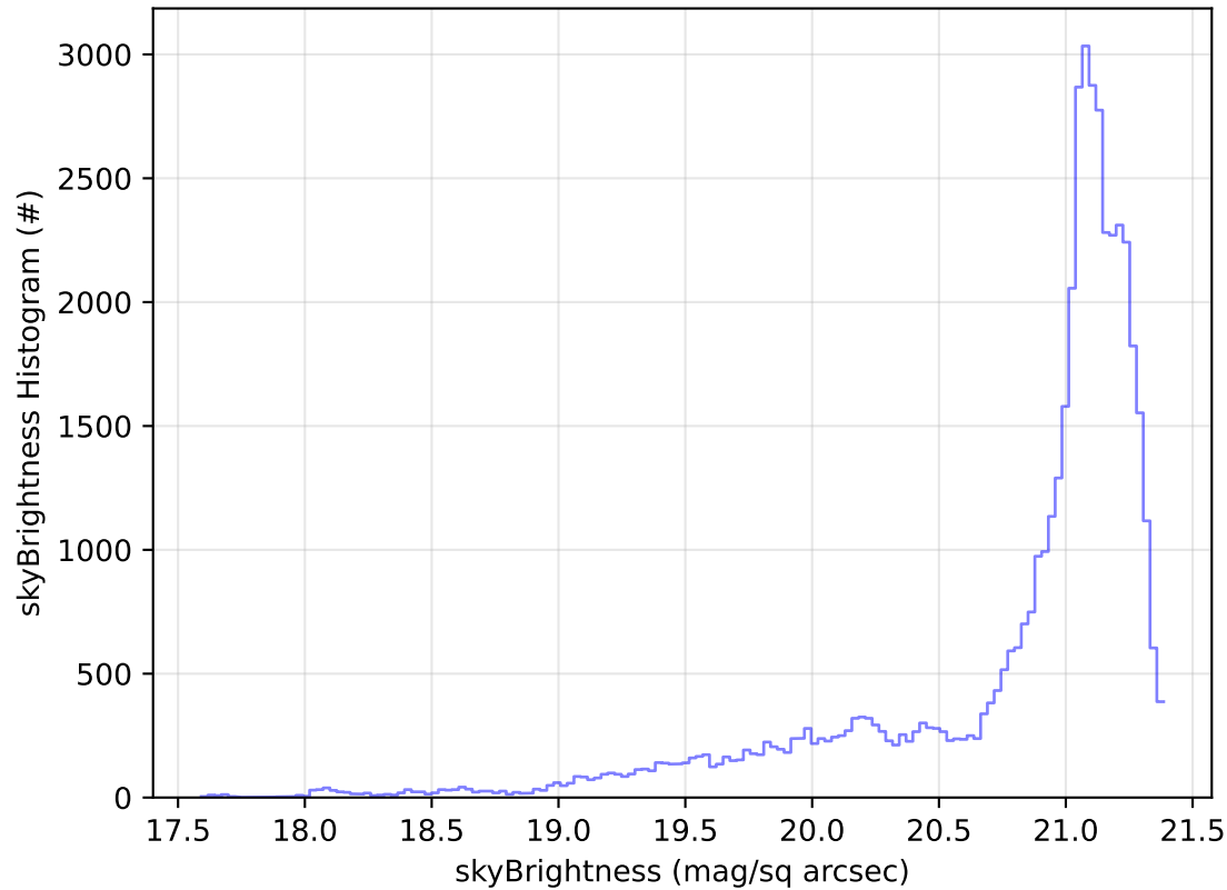
ddf_acor_sf10_lsf40_lsr20_v3.4_10yrs Yr 1 r band: skyBrightness Histogram
