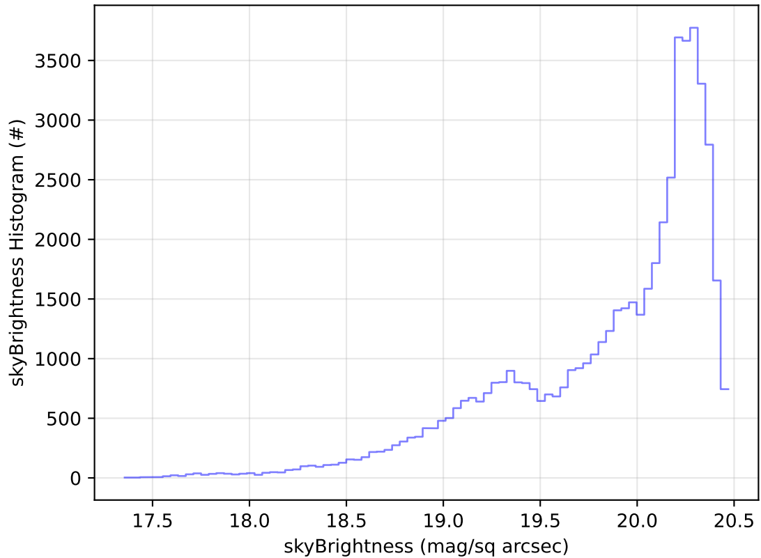
ddf_acor_sf10_lsf40_lsr20_v3.4_10yrs Yr 1 i band: skyBrightness Histogram
