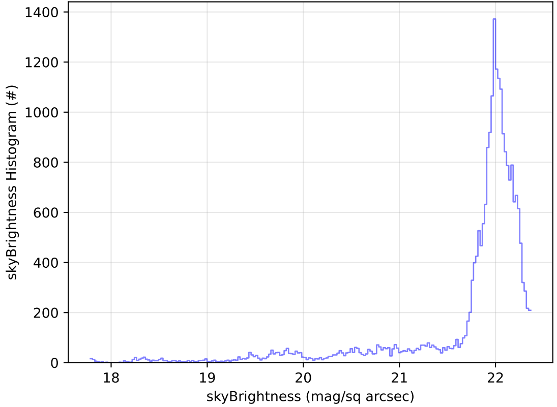
ddf_acor_sf10_lsf40_lsr20_v3.4_10yrs Yr 1 g band: skyBrightness Histogram
