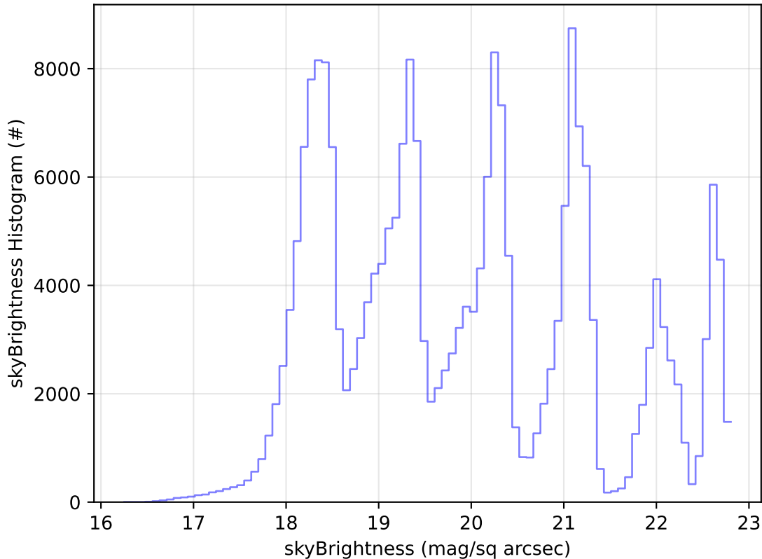
ddf_acor_sf10_lsf40_lsr20_v3.4_10yrs Yr 1 all bands: skyBrightness Histogram
