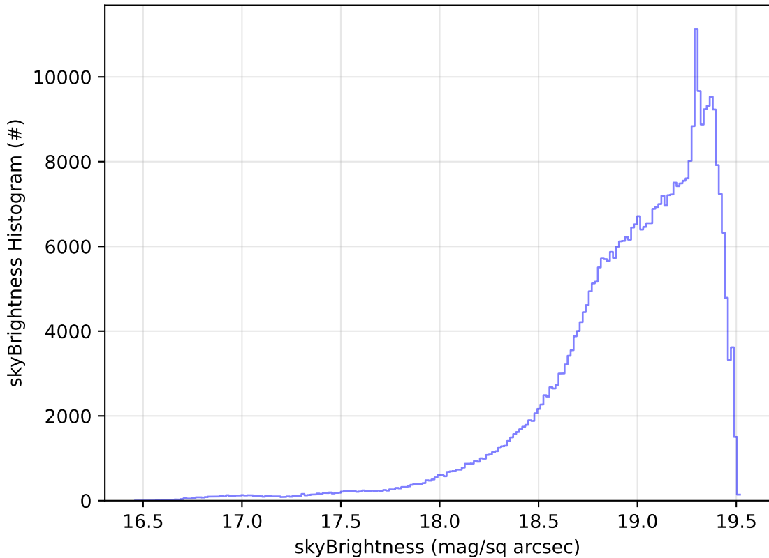
ddf_acor_sf10_lsf40_lsr20_v3.4_10yrs WFD z band: skyBrightness Histogram
