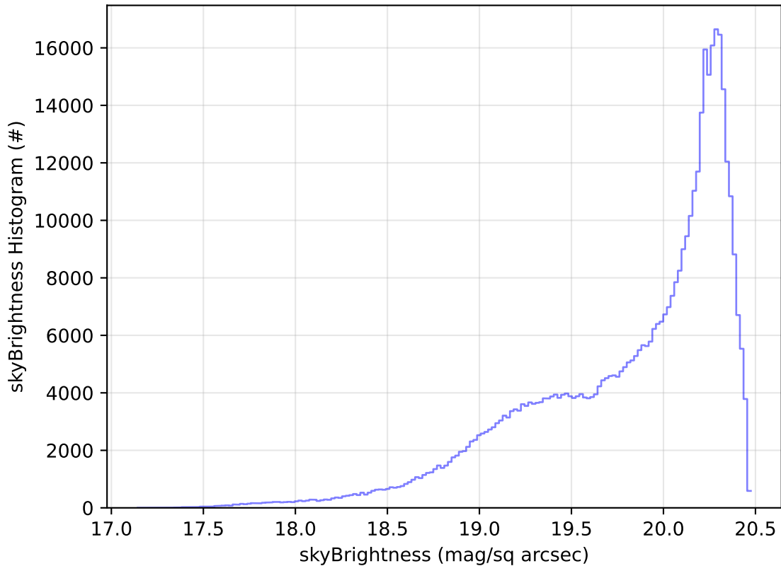
ddf_acor_sf10_lsf40_lsr20_v3.4_10yrs WFD i band: skyBrightness Histogram
