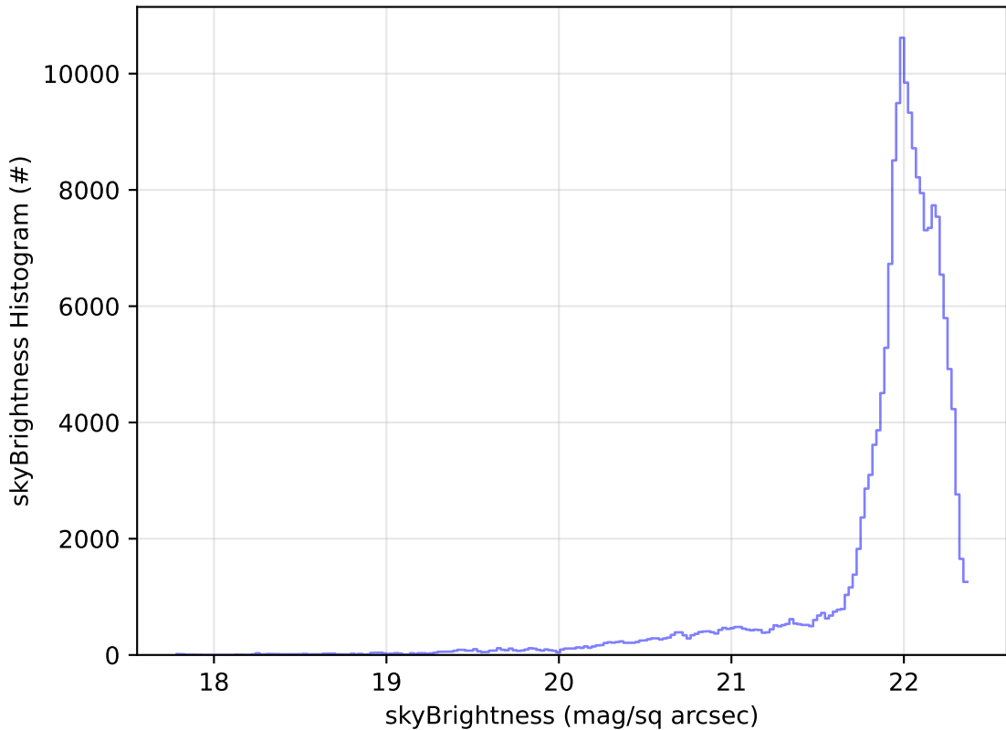
ddf_acor_sf10_lsf40_lsr20_v3.4_10yrs WFD g band: skyBrightness Histogram
