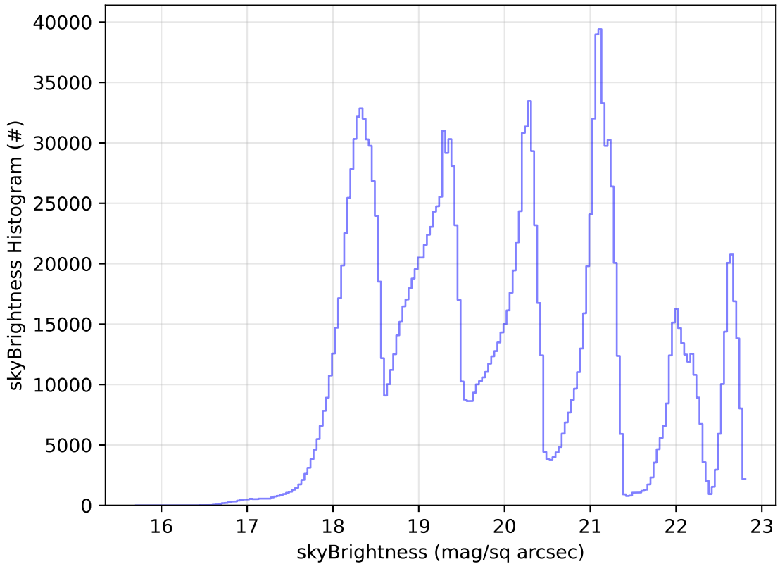
ddf_acor_sf10_lsf40_lsr20_v3.4_10yrs WFD all bands: skyBrightness Histogram
