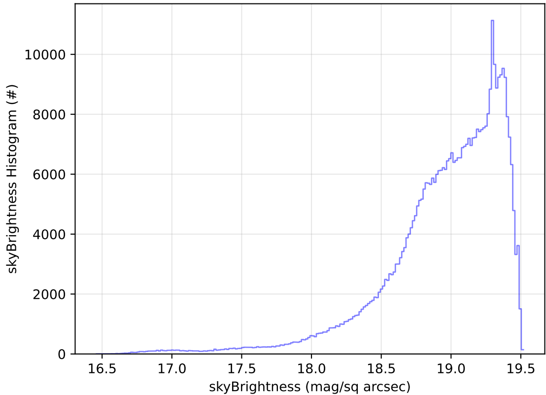
ddf_acor_sf10_lsf40_lsr20_v3.4_10yrs All sky z band: skyBrightness Histogram
