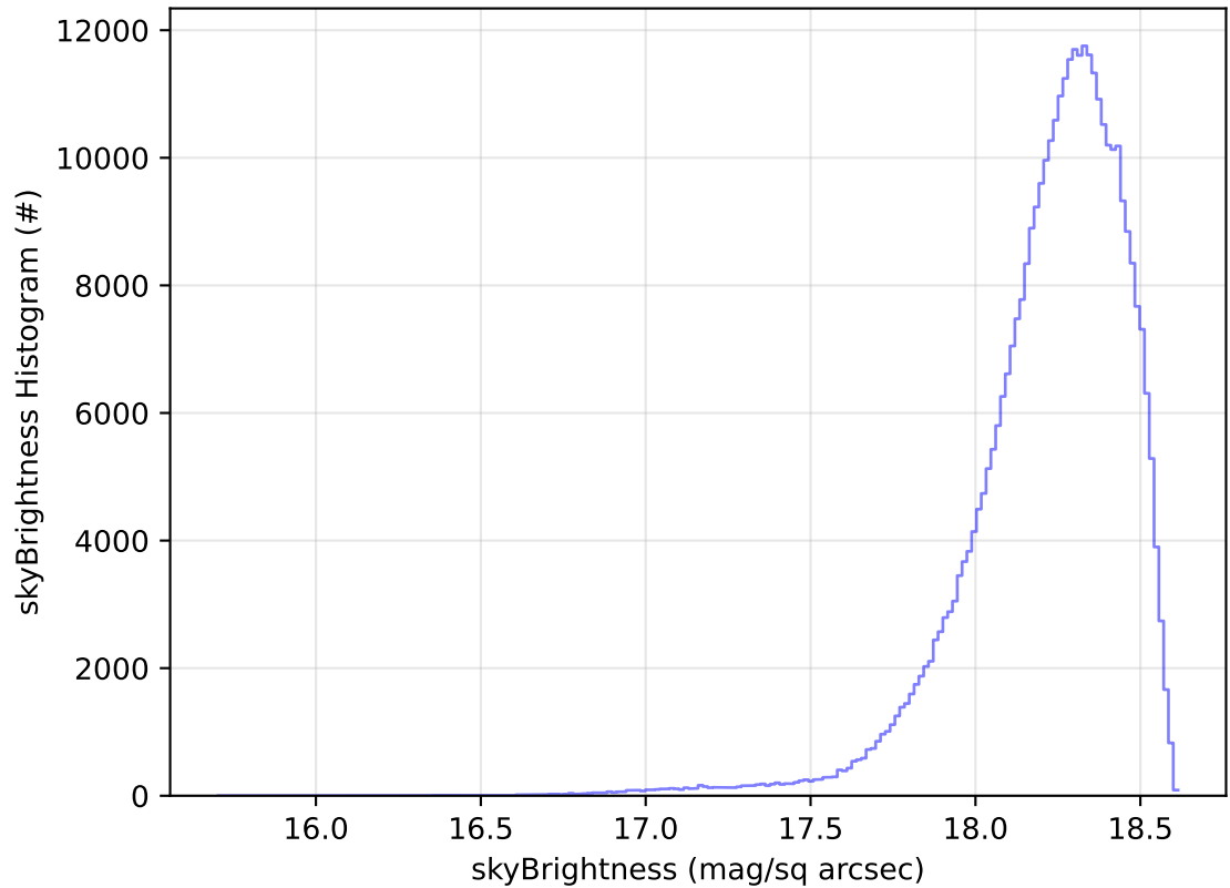
ddf_acor_sf10_lsf40_lsr20_v3.4_10yrs All sky y band: skyBrightness Histogram
