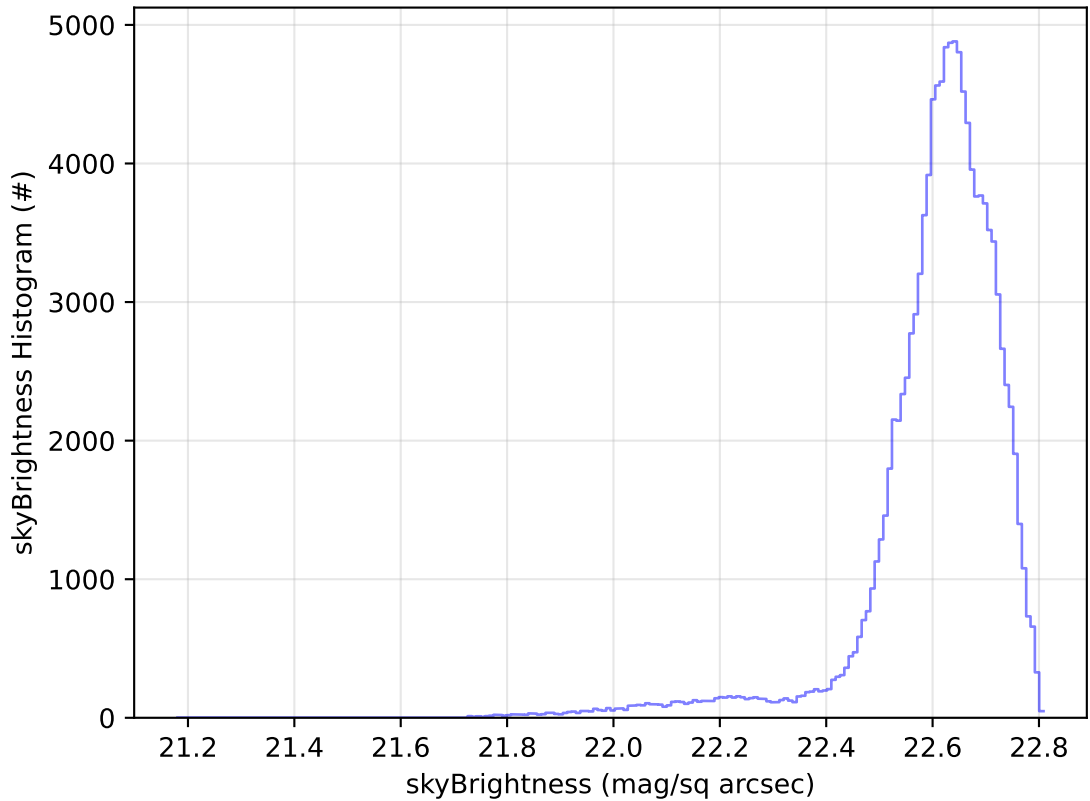
ddf_acor_sf10_lsf40_lsr20_v3.4_10yrs All sky u band: skyBrightness Histogram
