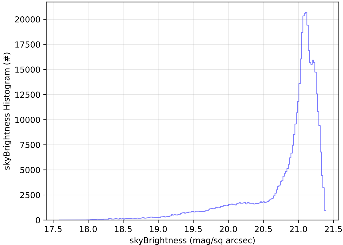
ddf_acor_sf10_lsf40_lsr20_v3.4_10yrs All sky r band: skyBrightness Histogram
