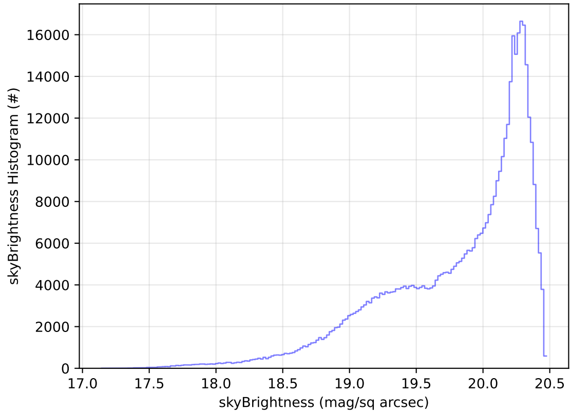
ddf_acor_sf10_lsf40_lsr20_v3.4_10yrs All sky i band: skyBrightness Histogram
