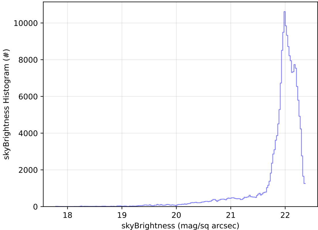
ddf_acor_sf10_lsf40_lsr20_v3.4_10yrs All sky g band: skyBrightness Histogram
