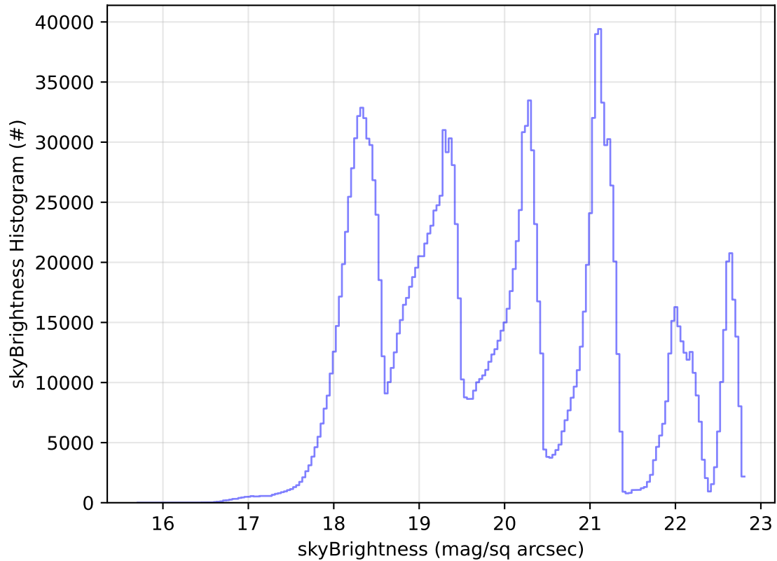
ddf_acor_sf10_lsf40_lsr20_v3.4_10yrs All sky all bands: skyBrightness Histogram
