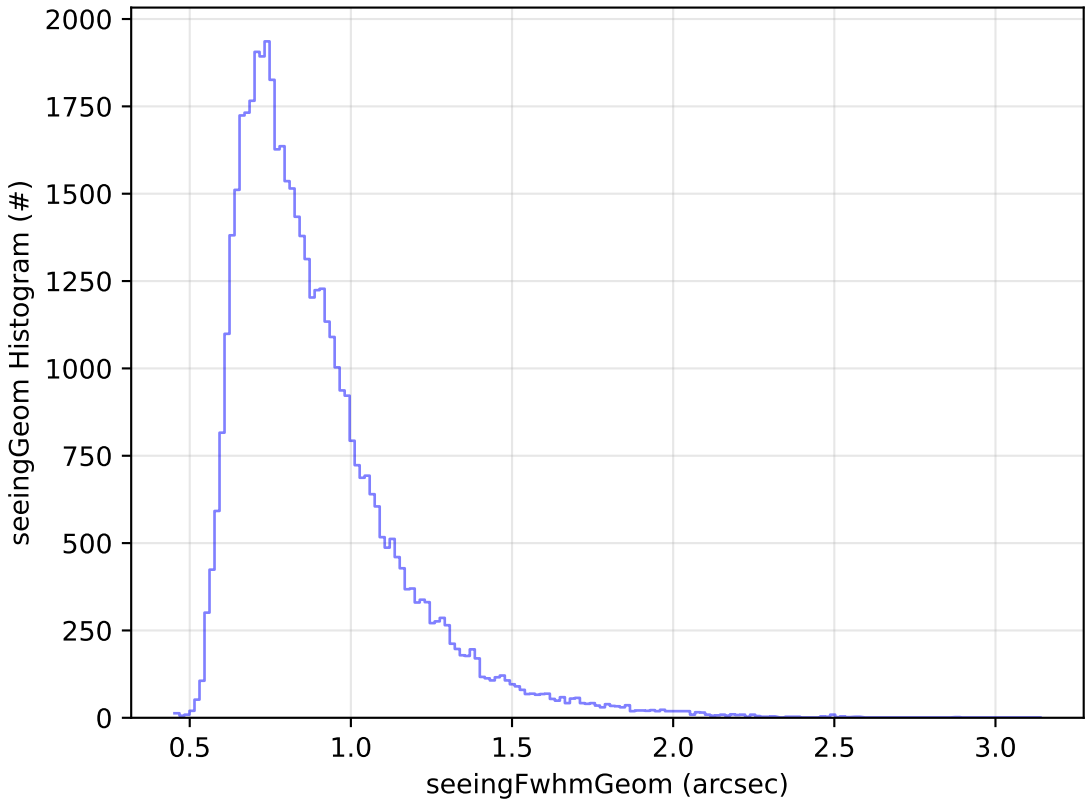
ddf_acor_sf10_lsf40_lsr20_v3.4_10yrs Yr 1 r band: seeingGeom Histogram
