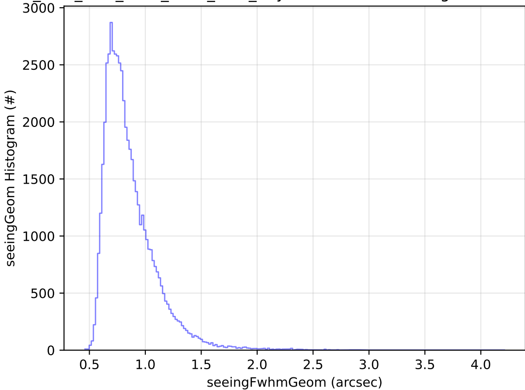
ddf_acor_sf10_lsf40_lsr20_v3.4_10yrs Yr 1 i band: seeingGeom Histogram
