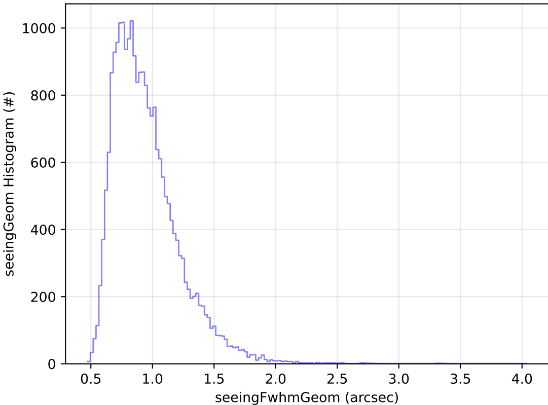
ddf_acor_sf10_lsf40_lsr20_v3.4_10yrs Yr 1 g band: seeingGeom Histogram
