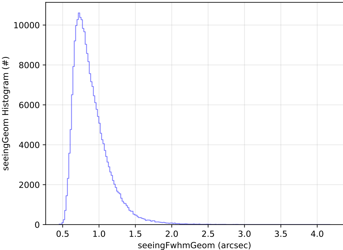
ddf_acor_sf10_lsf40_lsr20_v3.4_10yrs Yr 1 all bands: seeingGeom Histogram
