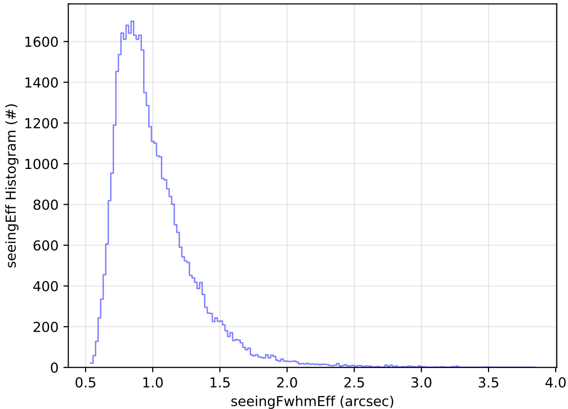
ddf_acor_sf10_lsf40_lsr20_v3.4_10yrs Yr 1 z band: seeingEff Histogram
