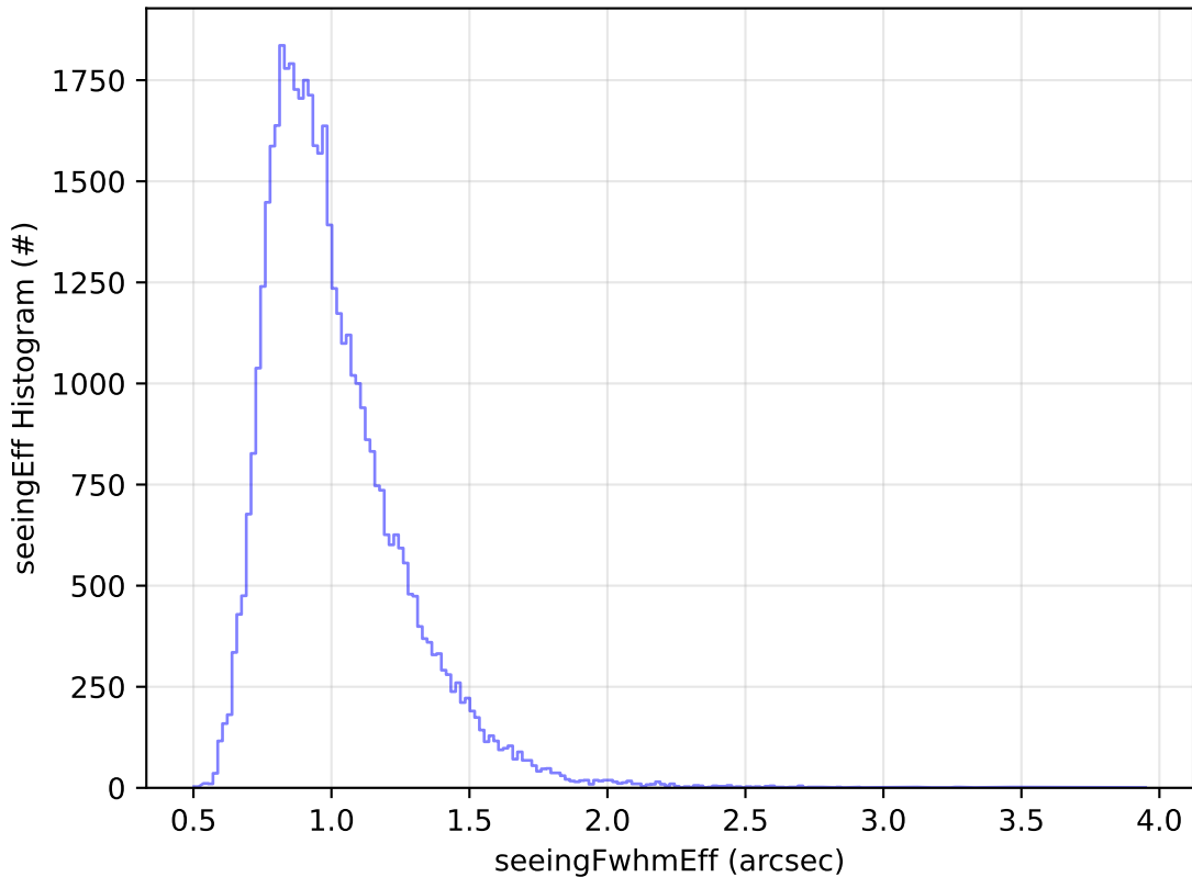
ddf_acor_sf10_lsf40_lsr20_v3.4_10yrs Yr 1 y band: seeingEff Histogram
