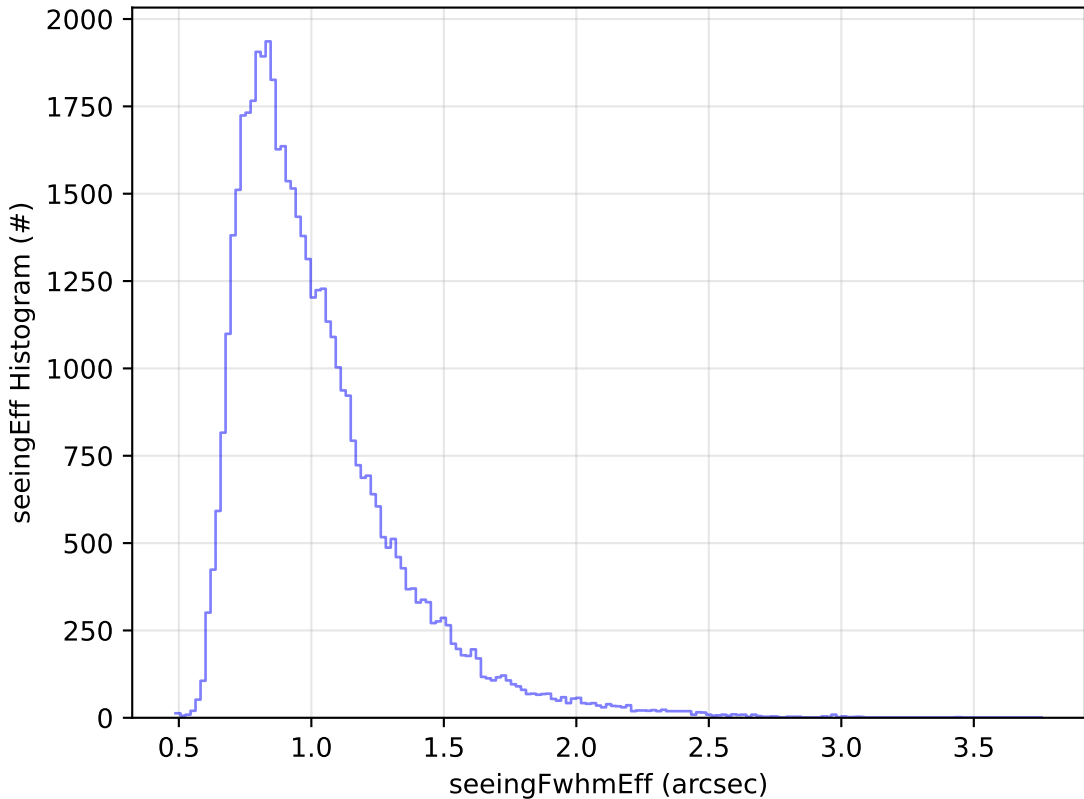
ddf_acor_sf10_lsf40_lsr20_v3.4_10yrs Yr 1 r band: seeingEff Histogram
