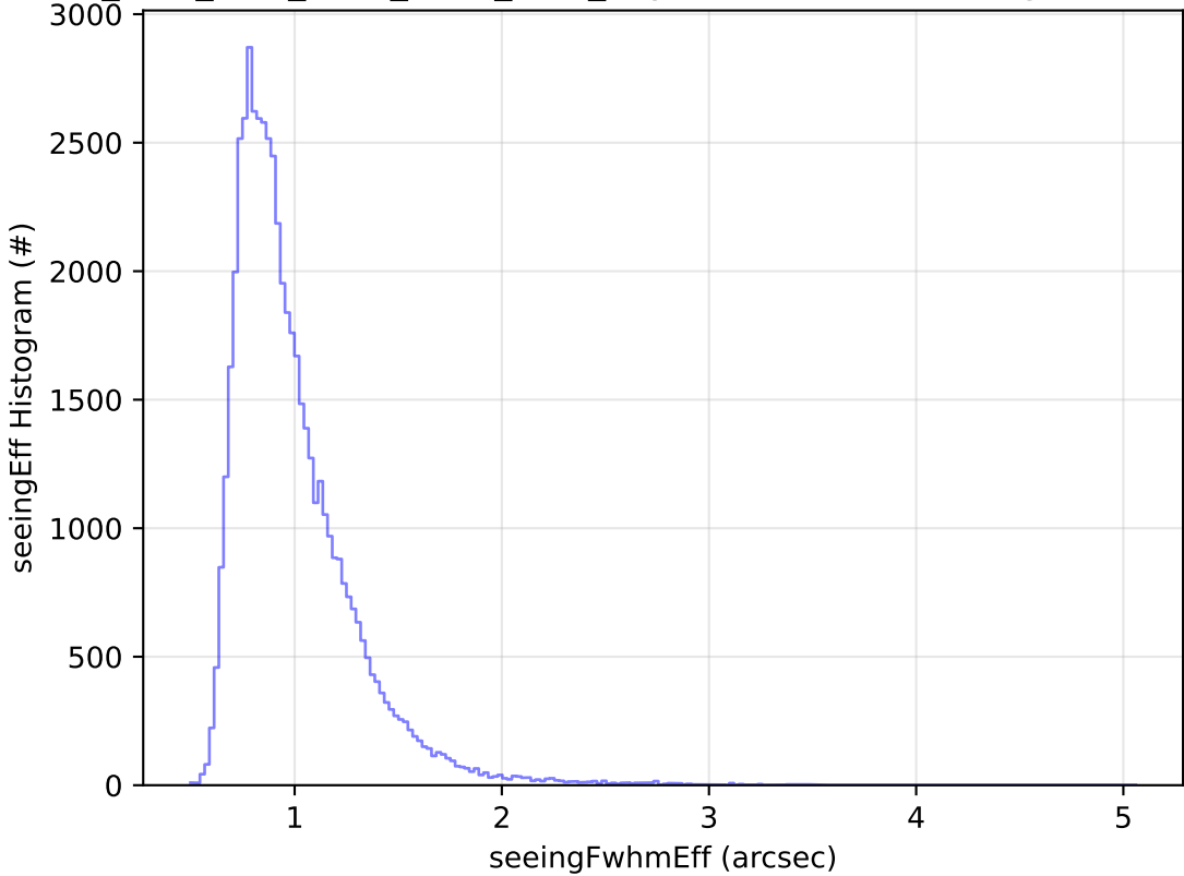
ddf_acor_sf10_lsf40_lsr20_v3.4_10yrs Yr 1 i band: seeingEff Histogram
