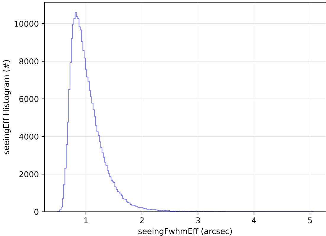
ddf_acor_sf10_Isf40_Isr20_v3.4_10yrs Yr 1 all bands: seeingEff Histogram
