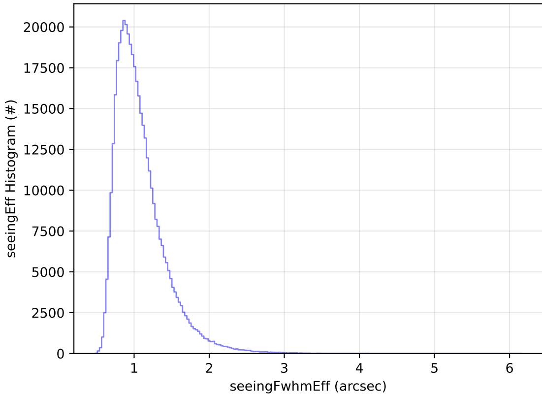
ddf_acor_sf10_lsf40_lsr20_v3.4_10yrs WFD z band: seeingEff Histogram
