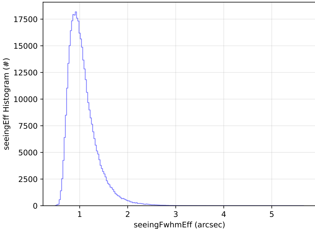
ddf_acor_sf10_lsf40_lsr20_v3.4_10yrs WFD y band: seeingEff Histogram
