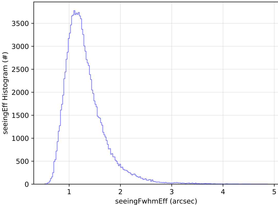
ddf_acor_sf10_lsf40_lsr20_v3.4_10yrs WFD u band: seeingEff Histogram
