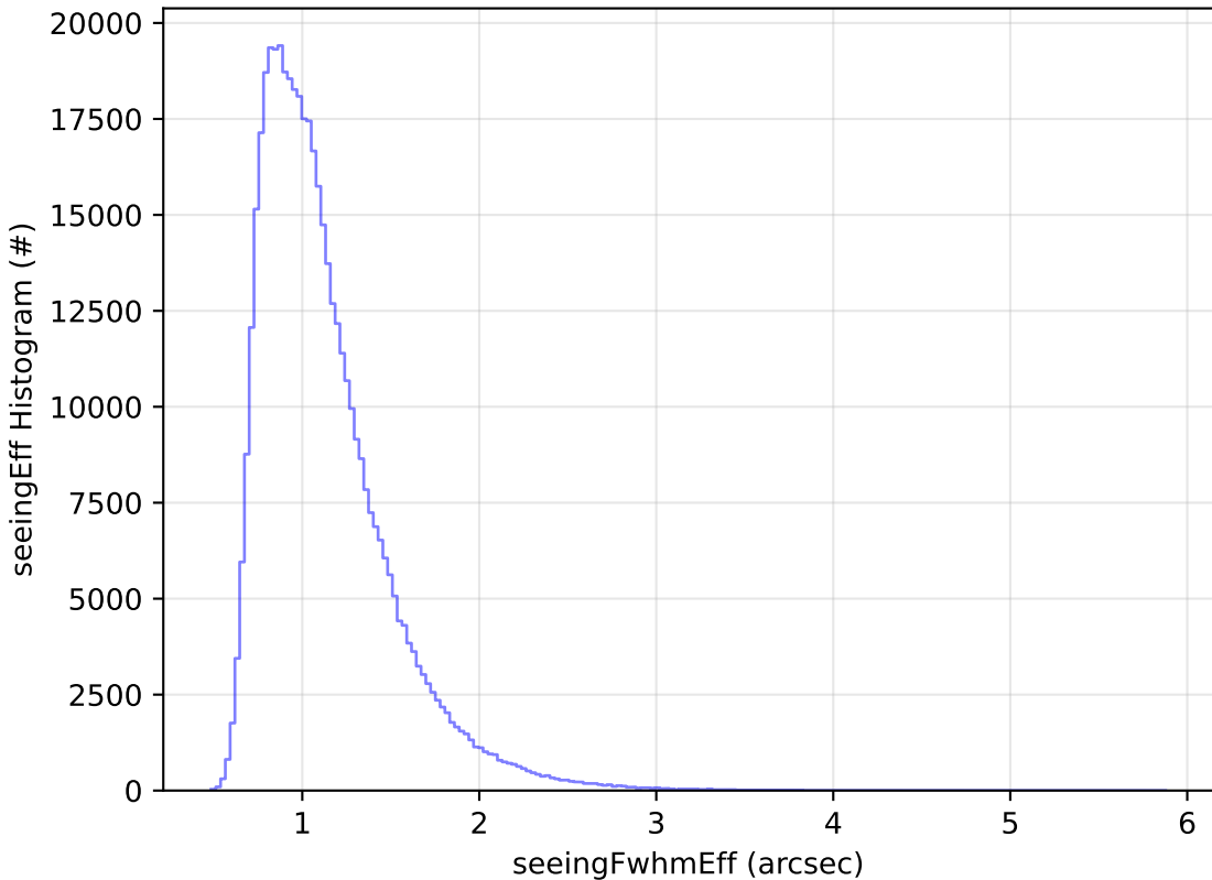
ddf_acor_sf10_lsf40_lsr20_v3.4_10yrs WFD r band: seeingEff Histogram
