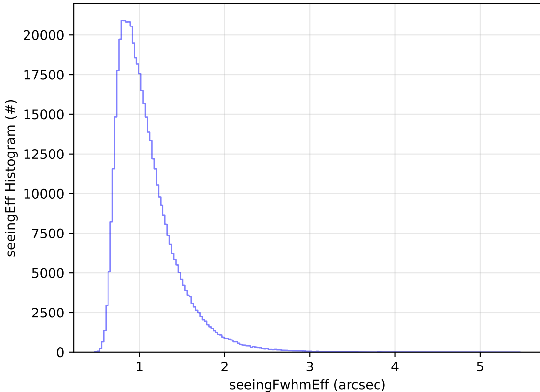
ddf_acor_sf10_lsf40_lsr20_v3.4_10yrs WFD i band: seeingEff Histogram
