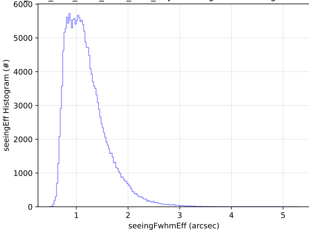
ddf_acor_sf10_lsf40_lsr20_v3.4_10yrs WFD g band: seeingEff Histogram
