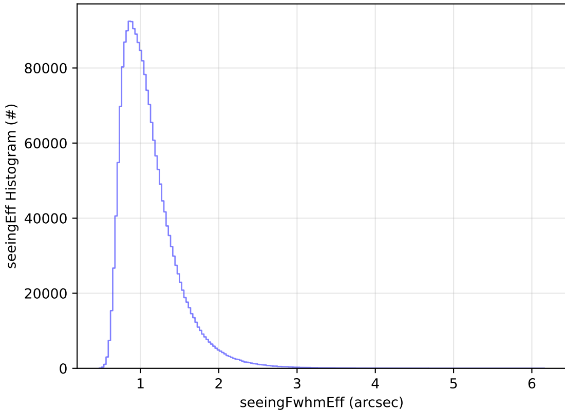
ddf_acor_sf10_lsf40_lsr20_v3.4_10yrs WFD all bands: seeingEff Histogram
