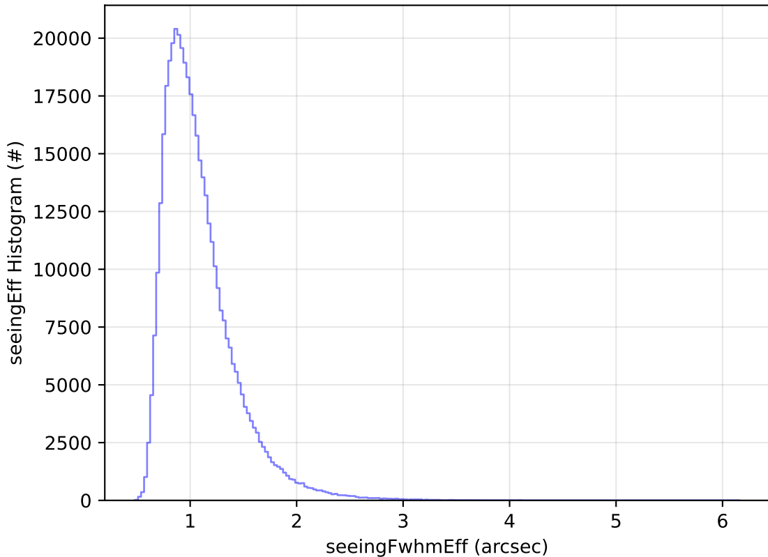
ddf_acor_sf10_lsf40_lsr20_v3.4_10yrs All sky z band: seeingEff Histogram
