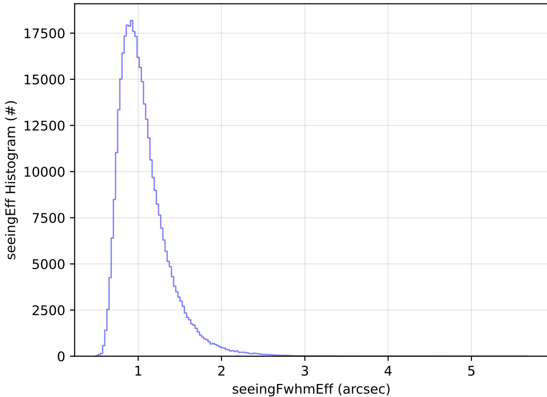
ddf_acor_sf10_lsf40_lsr20_v3.4_10yrs All sky y band: seeingEff Histogram
