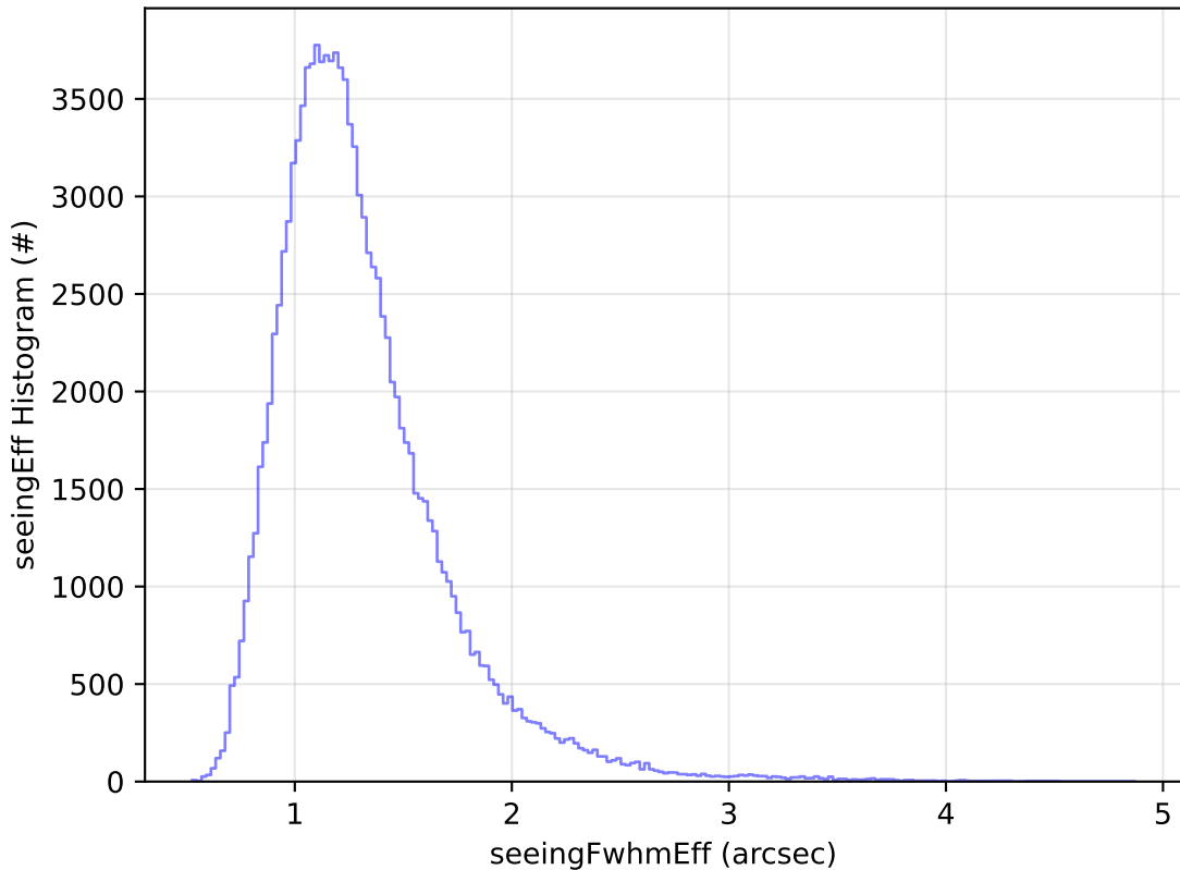
ddf_acor_sf10_ls40_lsr20_v3.4_10yrs All sky u band: seeingEff Histogram
