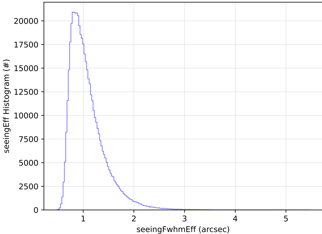
ddf_acor_sf10_lsf40_lsr20_v3.4_10yrs All sky i band: seeingEff Histogram
