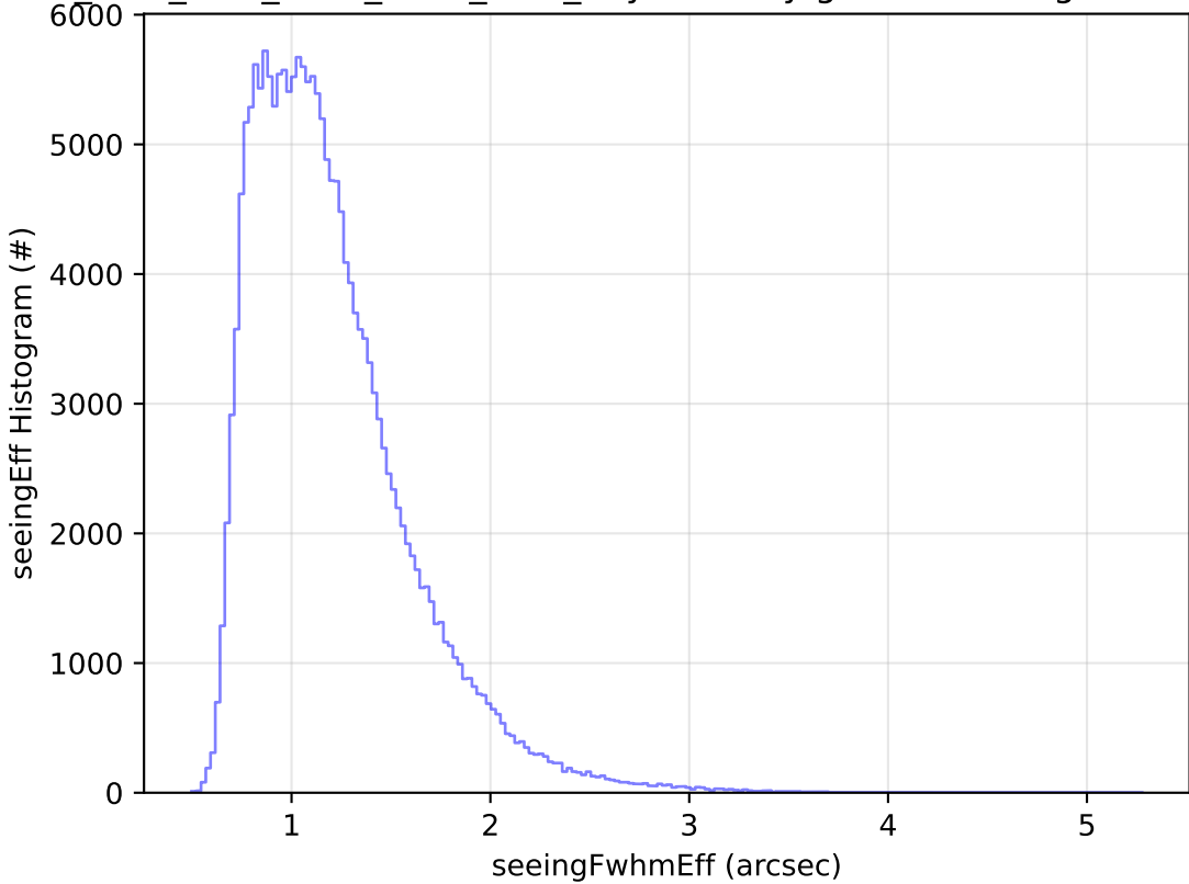
ddf_acor_sf10_lsf40_lsr20_v3.4_10yrs All sky g band: seeingEff Histogram
