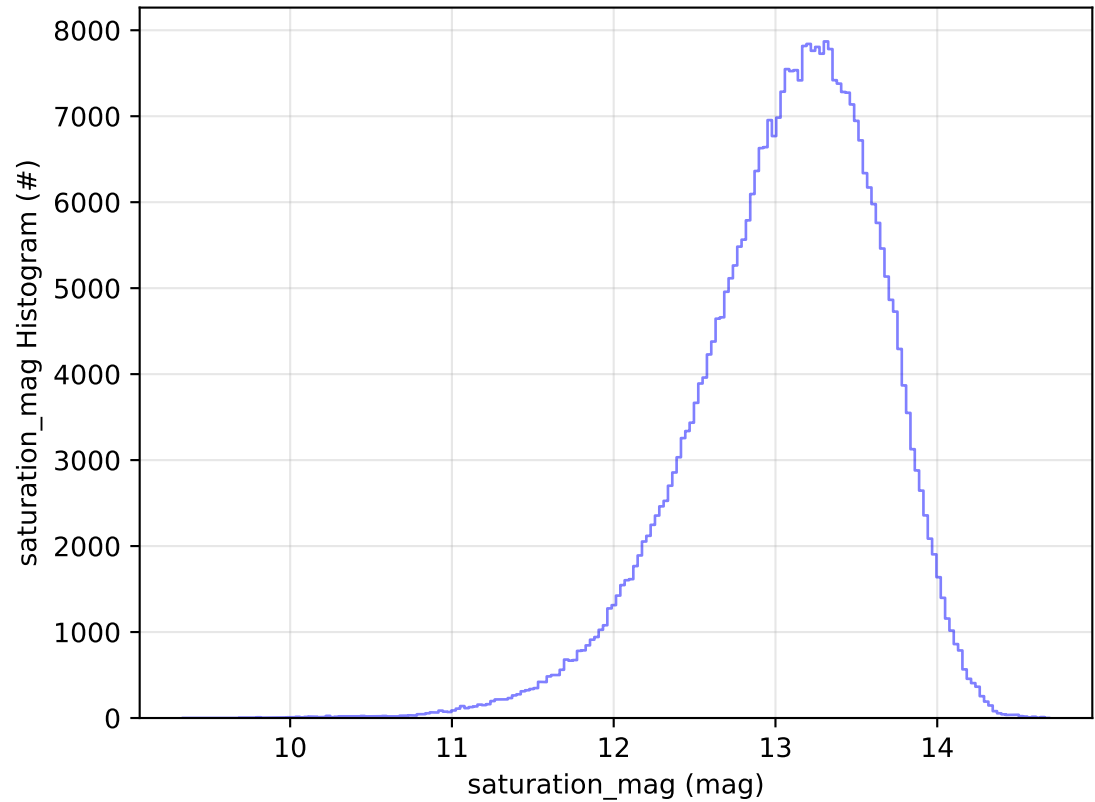
ddf_acor_sf10_lsf40_lsr20_v3.4_10yrs WFD y band: saturation_mag Histogram
