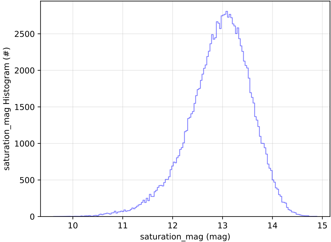
ddf_acor_sf10_lsf40_lsr20_v3.4_10yrs WFD u band: saturation_mag Histogram
