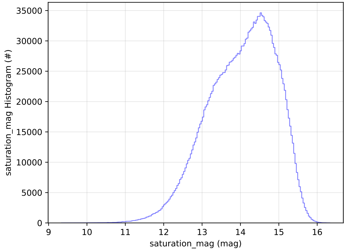
ddf_acor_sf10_lsf40_lsr20_v3.4_10yrs WFD all bands: saturation_mag Histogram
