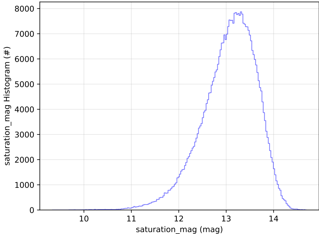
ddf_acor_sf10_lsf40_lsr20_v3.4_10yrs All sky y band: saturation_mag Histogram
