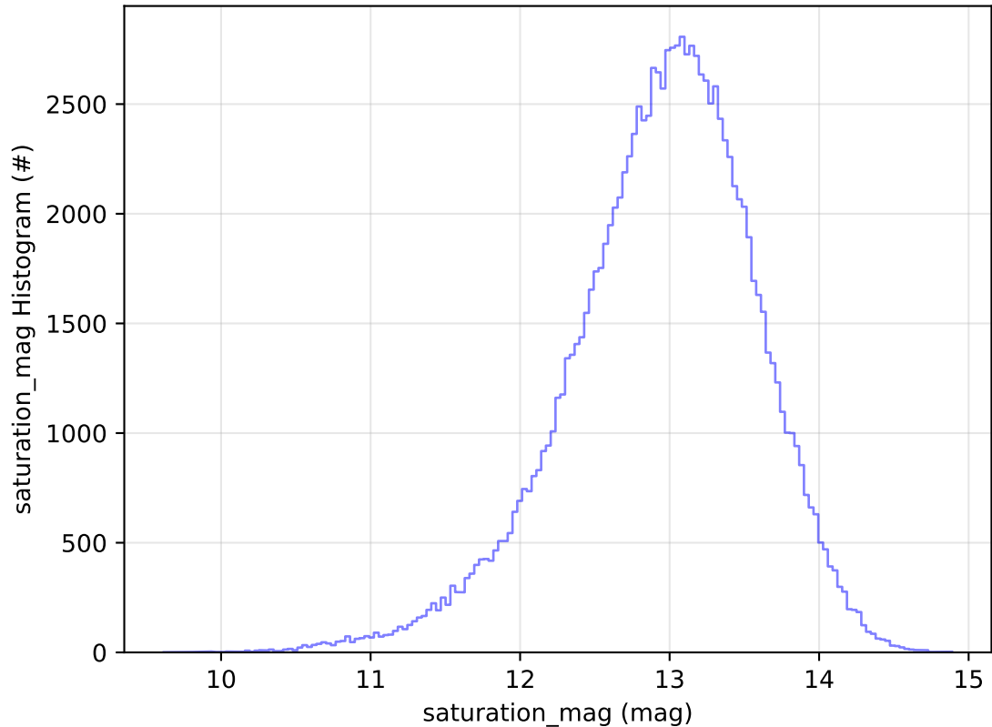
ddf_acor_sf10_lsf40_lsr20_v3.4_10yrs All sky u band: saturation_mag Histogram
