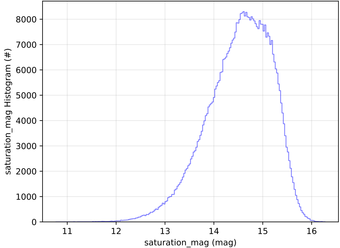
ddf_acor_sf10_lsf40_lsr20_v3.4_10yrs All sky r band: saturation_mag Histogram
