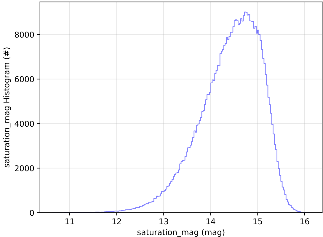
ddf_acor_sf10_lsf40_lsr20_v3.4_10yrs All sky i band: saturation_mag Histogram
