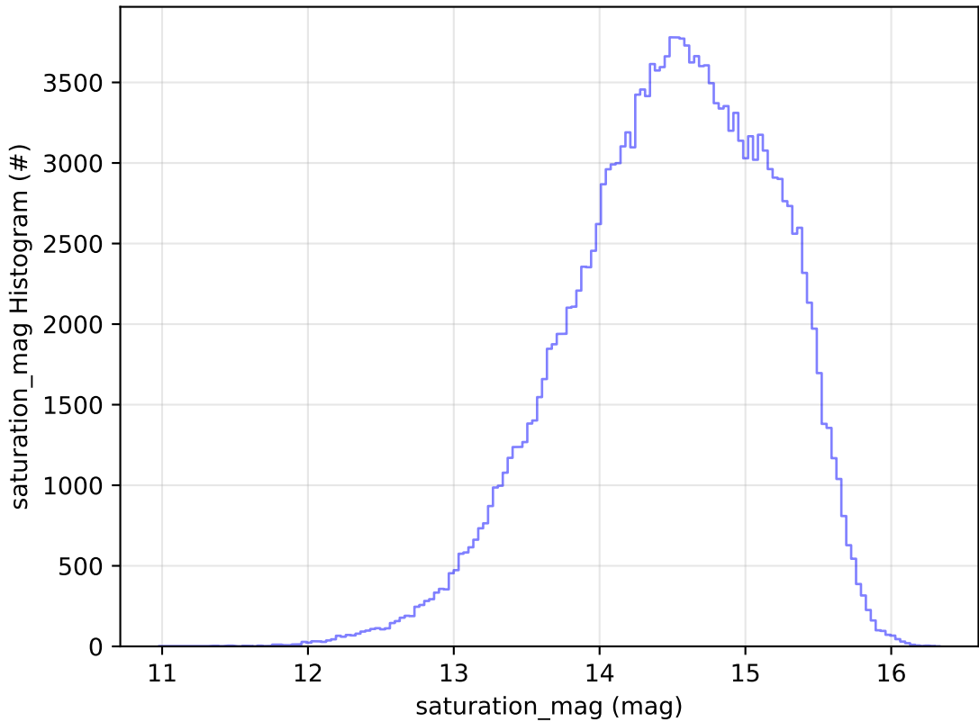
ddf_acor_sf10_lsf40_lsr20_v3.4_10yrs All sky g band: saturation_mag Histogram
