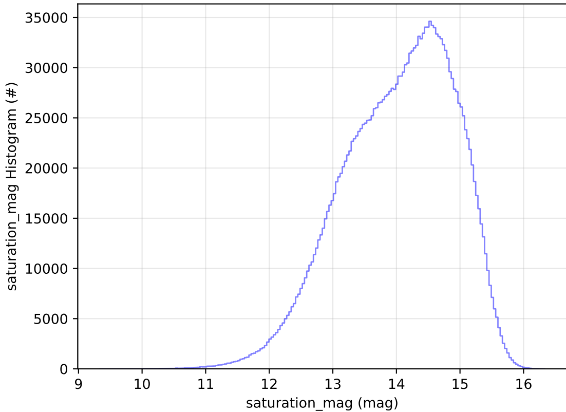
ddf_acor_sf10_lsf40_lsr20_v3.4_10yrs All sky all bands: saturation_mag Histogram
