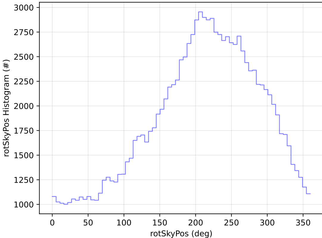
ddf_acor_sf10_lsf40_lsr20_v3.4_10yrs WFD u band: rotSkyPos Histogram
