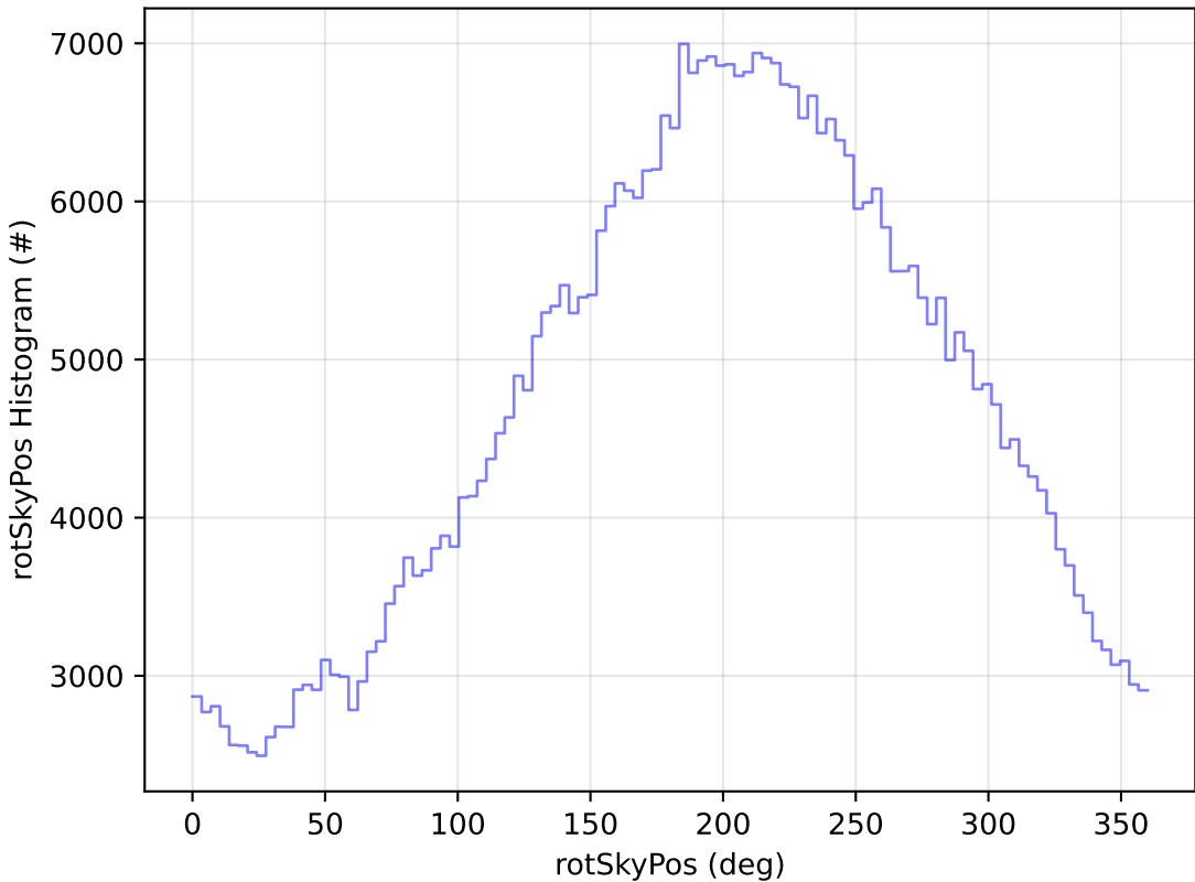
ddf_acor_sf10_lsf40_lsr20_v3.4_10yrs WFD r band: rotSkyPos Histogram
