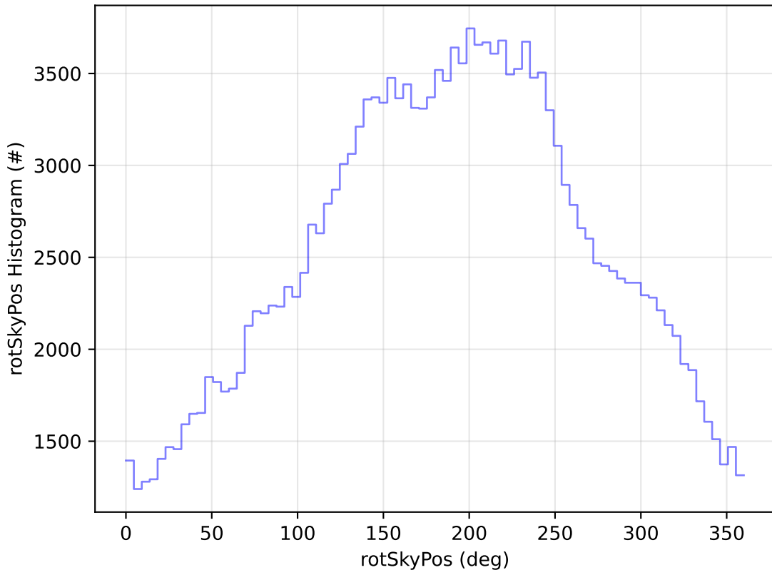
ddf_acor_sf10_lsf40_lsr20_v3.4_10yrs WFD g band: rotSkyPos Histogram
