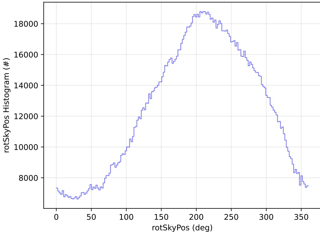
ddf_acor_sf10_ls40_lsr20_v3.4_10yrs WFD all bands: rotSkyPos Histogram
